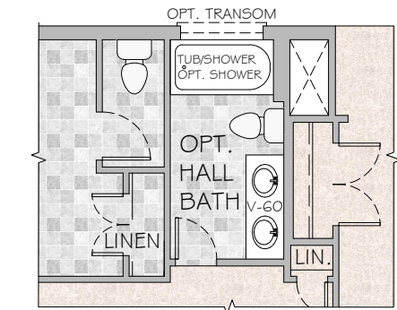
OPTIONAL HALL BATH LAYOUT
