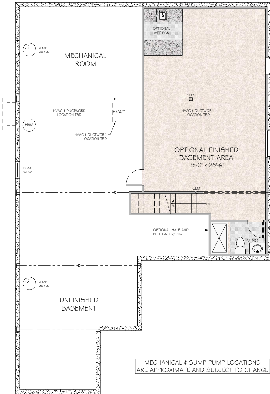
OPTIONAL FINISHED BASEMENT PLAN
