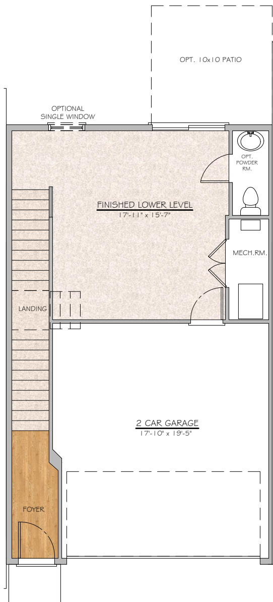
DEWEY LOWER LEVEL PLAN
